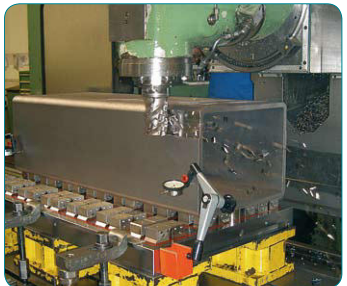
QX HD 50 with pole extensions for working with low vibrations
