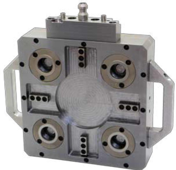
RS Magnet circular chuck with System Erowa ITS
